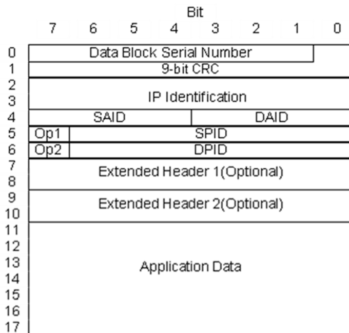
Figure 5.17: Confirmed rate ¾ coded data with UDP/IPv4 Header Compression
