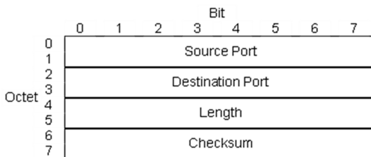
Figure 5.14: UDP Header
