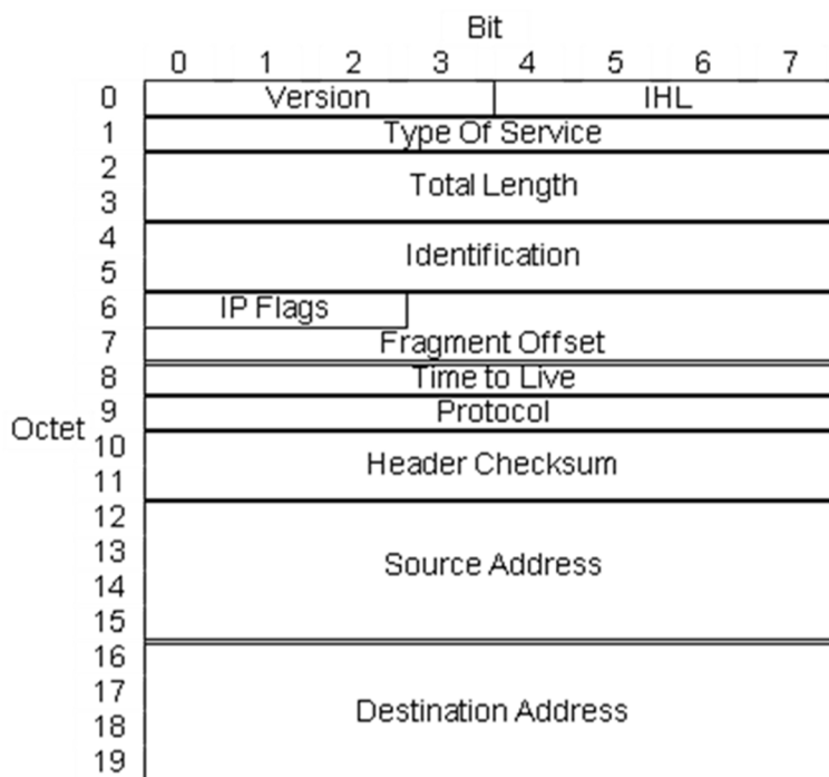
Figure 5.15: IPv4 Header
